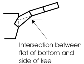
d) Vessel with hollow garboards
