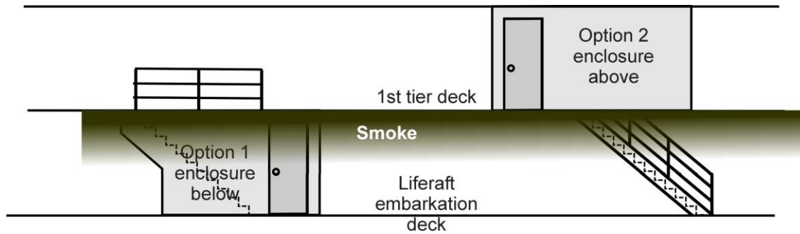
Figure 8 — Stairs penetrating 2 decks
