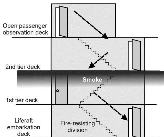
Figure 9— Stairway tower penetrating 3 or more decks
