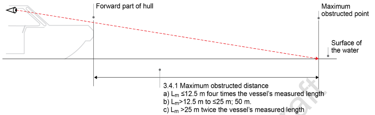
Figure 3 — Field of vision from the operating station (clause 3.4)
