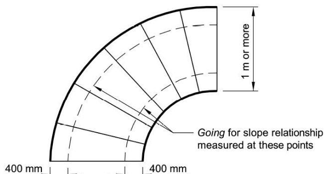
Tapered treads — 1 m or more in width
