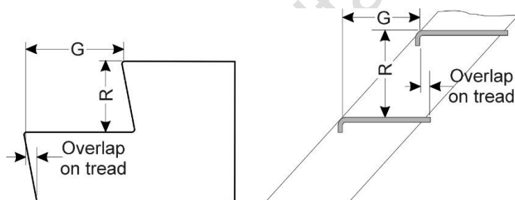
Figure 8 - Dimensions of steps in stairways
